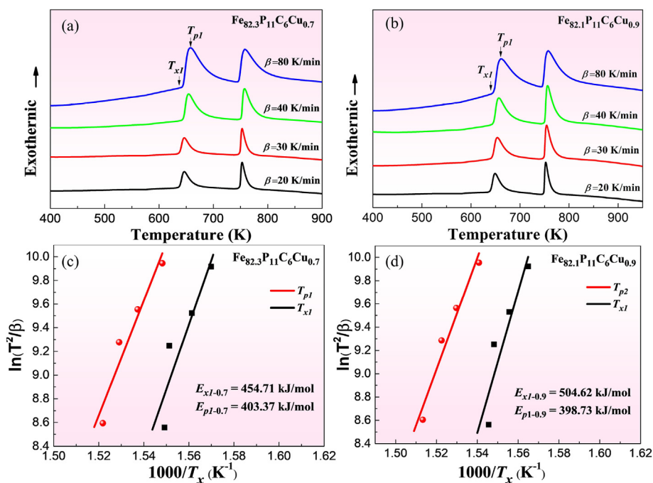
Fig. 5. (a–b) DSC curves of \text{Fe}_{83-x}\text{P}_{11}\text{C}_6\text{Cu}_x ( x = 0.7 and 0.9 at. %) ribbons at different heating rates (20, 30, 40, and 80 K/min) (c–d) Kissinger plots of \text{Fe}_{83-x}\text{P}_{11}\text{C}_6\text{Cu}_x ( x = 0.7 and 0.9 at. %) ribbons, symbols are experimental data, lines are fitting results.
