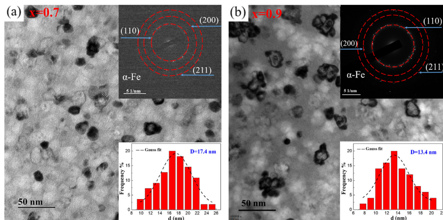
Fig. 4. TEM images of \text{Fe}_{83-x}\text{P}_{11}\text{C}_6\text{Cu}_x ((a) x = 0.7 and (b) 0.9 at. %) alloys annealed at T_{x2} -50 K, the illustrations are SAED patterns and grain size distribution, respectively.
