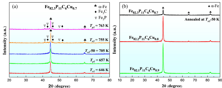
Fig. 3. (a) XRD patterns of \text{Fe}_{82.3}\text{P}_{11}\text{C}_6\text{Cu}_{0.7} amorphous ribbon annealed at different temperatures for 5 min (b) XRD patterns of \text{Fe}_{83-x}\text{P}_{11}\text{C}_6\text{Cu}_x ( x = 0.7, 0.8 and 0.9 at. %) amorphous ribbons annealed at T_{x2}-50 K for 5 min.
