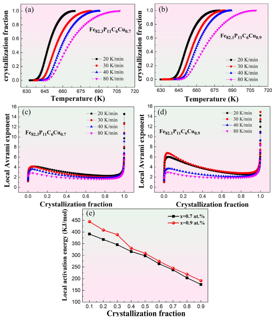
Fig. 6. (a–b) Crystallization fraction as a function of temperature for Fe 83–x P 11 C 6 Cu x (x = 0.7 and 0.9 at. %) alloys at different heating rates (c–d) The local Avrami exponent on the crystallization fraction (e) The relationship between local activation energy and crystallization fraction.
