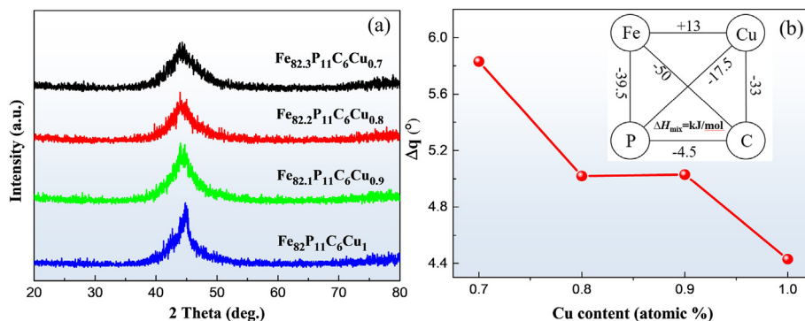
Fig. 1. (a) The XRD patterns of \text{Fe}_{83-x}\text{P}_{11}\text{C}_6\text{Cu}_x ( x = 0.7\text{--}1.0 at. %) as-spun ribbons (b) \Delta q of XRD patterns as a function of Cu content.
