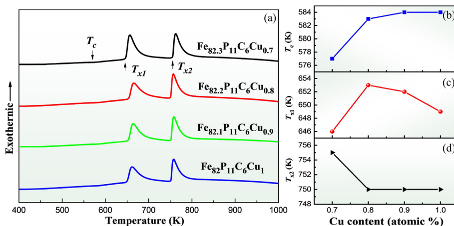
Fig. 2. (a) The DSC curves of \text{Fe}_{83-x}\text{P}_{11}\text{C}_6\text{Cu}_x ( x = 0.7\text{--}1.0 at. %) amorphous ribbons at a heating rate of 0.67 K/s (b–d) The Curie temperature T_c and two crystallization onset temperature T_{x1} and T_{x2} as a function of Cu content.
