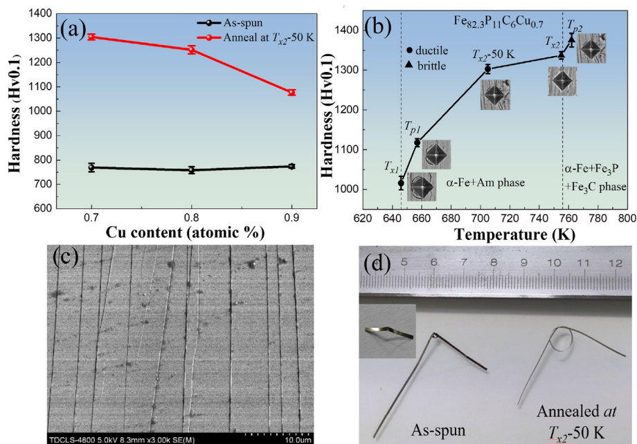
Fig. 8. (a) The relationship between Vickers hardness ( H_v ) and Cu content of Fe 83-x P 11 C 6 Cu x ( x = 0.7, 0.8 and 0.9 at. %) amorphous alloy in as-spun state and annealing at T_{x2} -50 K (b) Changes in H_v with annealing temperatures of Fe 82.3 P 11 C 6 Cu 0.7 ribbon (c) SEM images of the curved outer surface of Fe 82.3 P 11 C 6 Cu 0.7 as-spun ribbon (d) Bending ductility test of Fe 82.3 P 11 C 6 Cu 0.7 amorphous alloy after as-spun and T_{x2} -50 K annealing.
