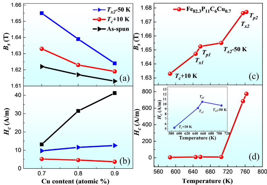
Fig. 7. (a–b) Changes in B_s and H_c with Cu contents of \text{Fe}_{83-x}\text{P}_{11}\text{C}_6\text{Cu}_x ( x = 0.7, 0.8 and 0.9 at. %) ribbons in as-spun, annealed T_c + 10 K and T_{x2}=50 K for 5 min (c–d) Changes in B_s and H_c with annealing temperatures of \text{Fe}_{82.3}\text{P}_{11}\text{C}_6\text{Cu}_{0.7} ribbon, the illustrations are enlarged image of H_c before 720 K.
